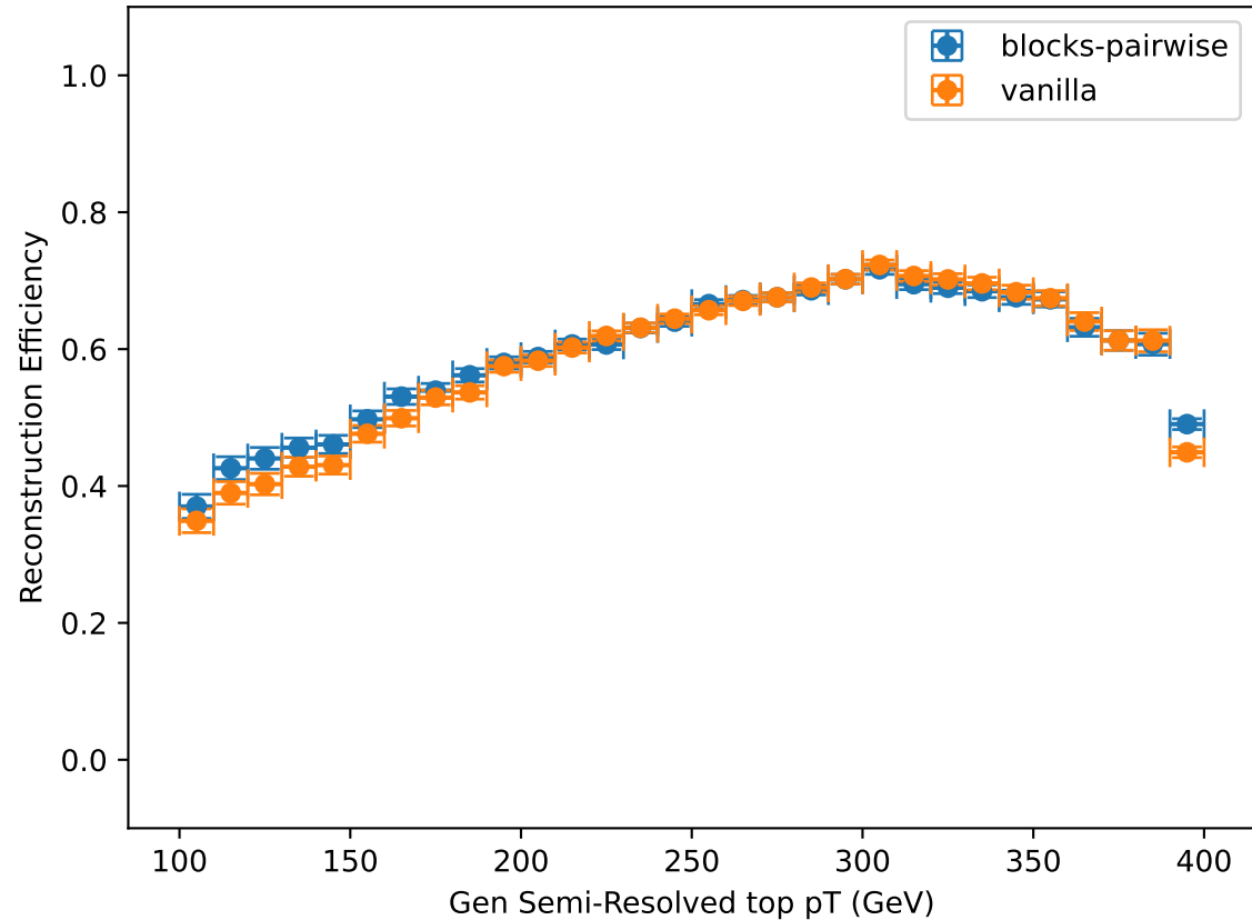
Reconstruction Efficiency vs. Gen Semi-Resolved top pT
