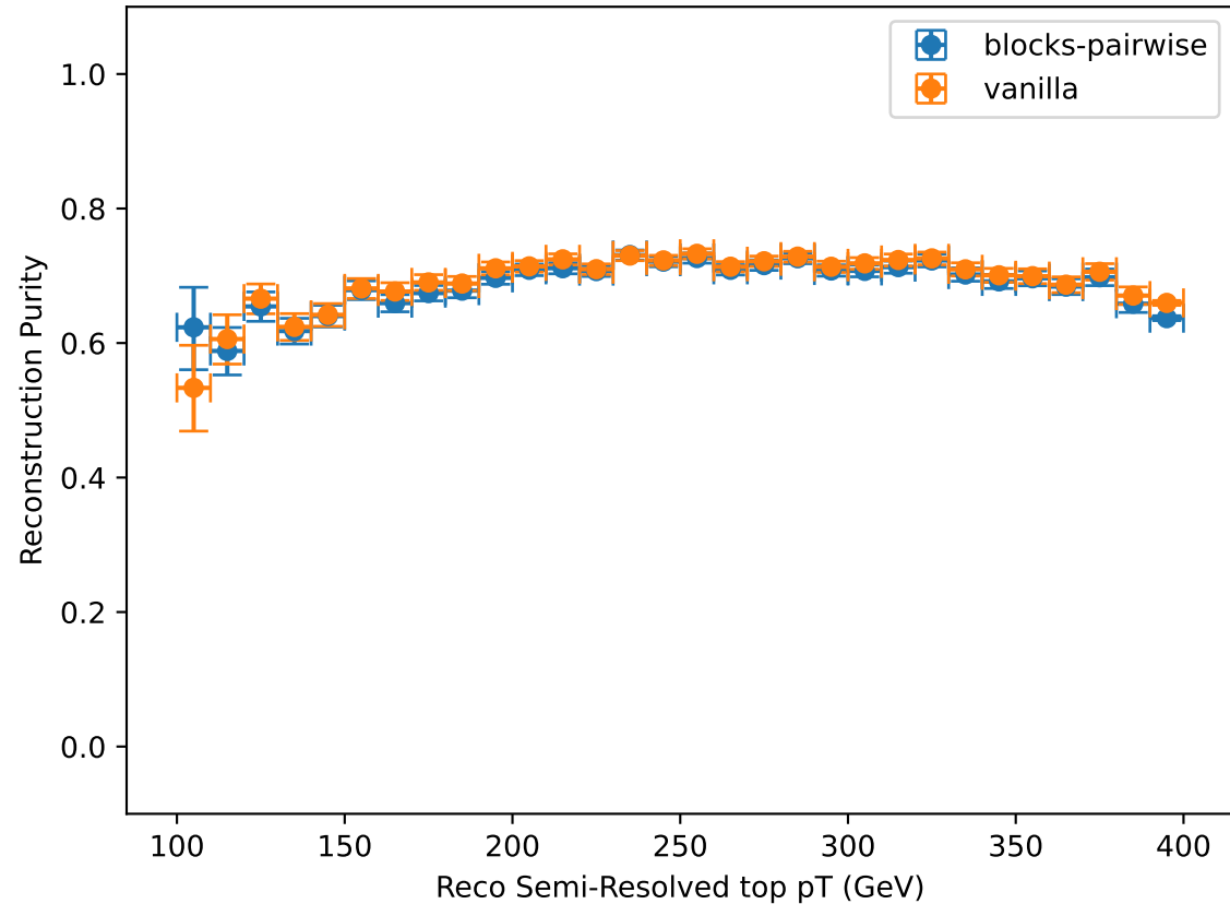
Reconstruction Purity vs. Reco Semi-Resolved top pT
