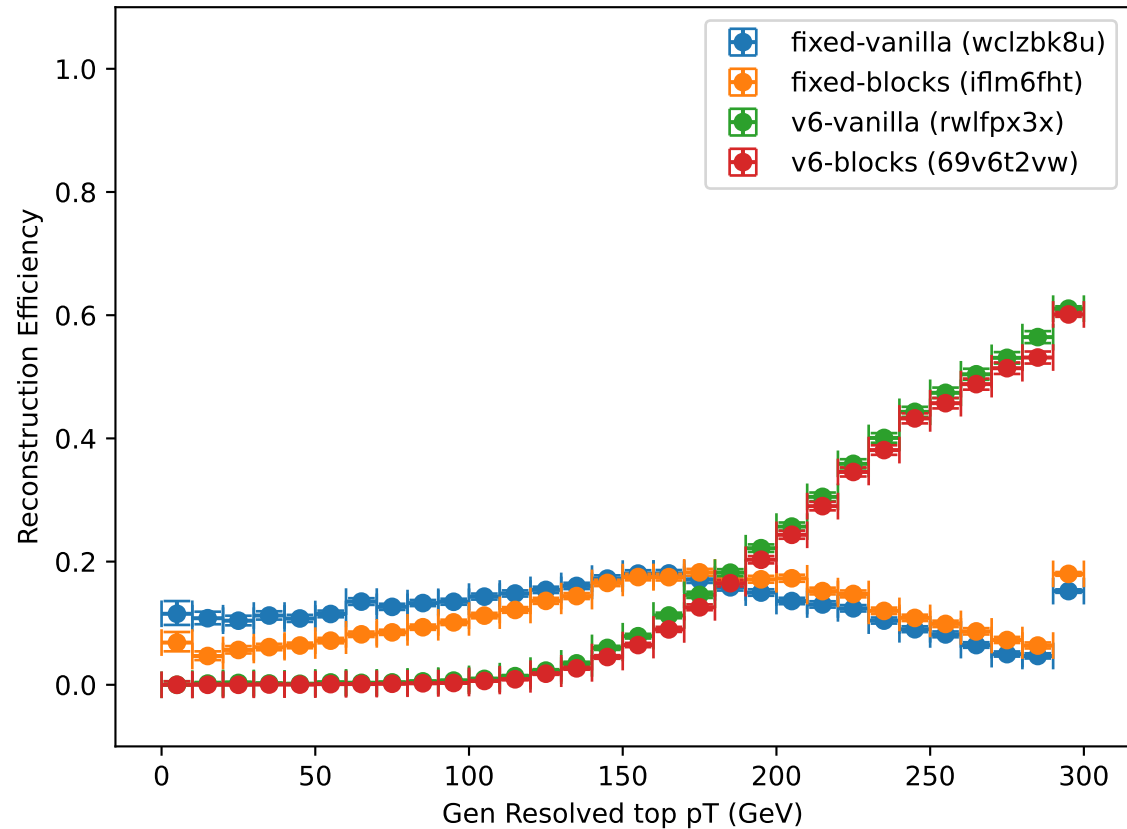
Reconstruction Efficiency vs. Gen Resolved top pT
