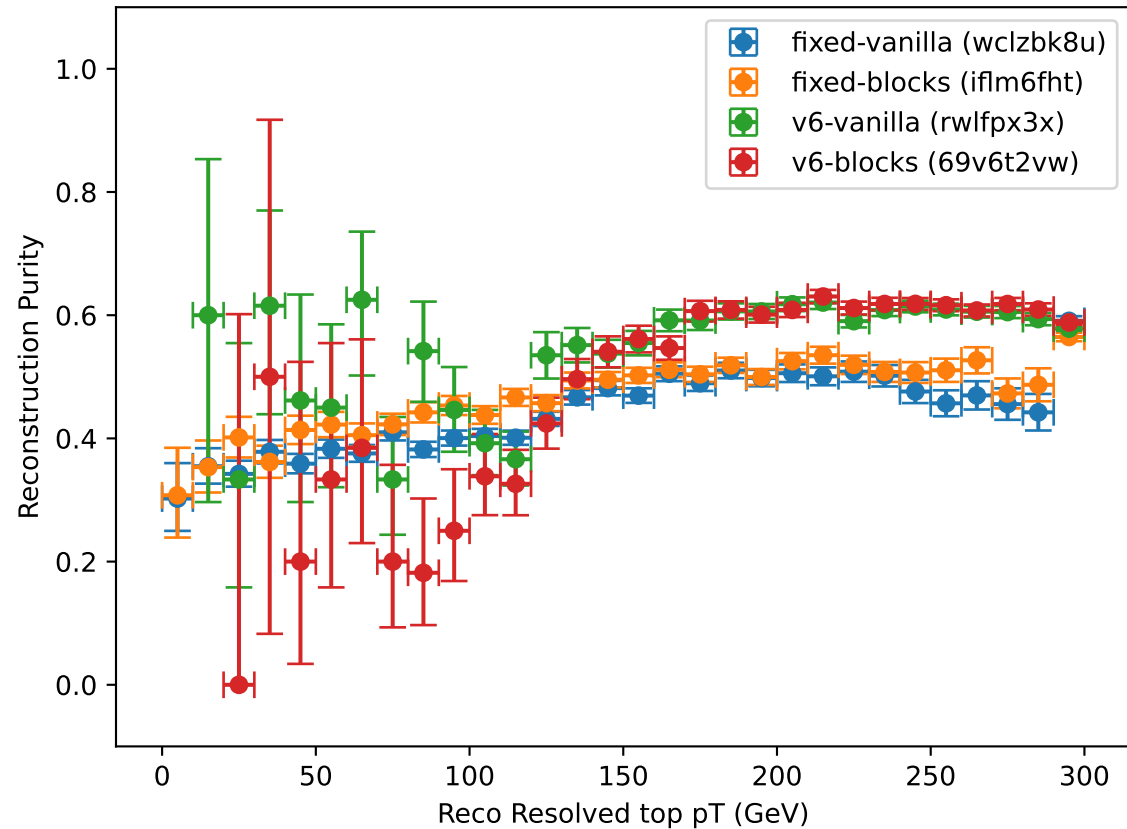
Reconstruction Purity vs. Reco Resolved top pT
