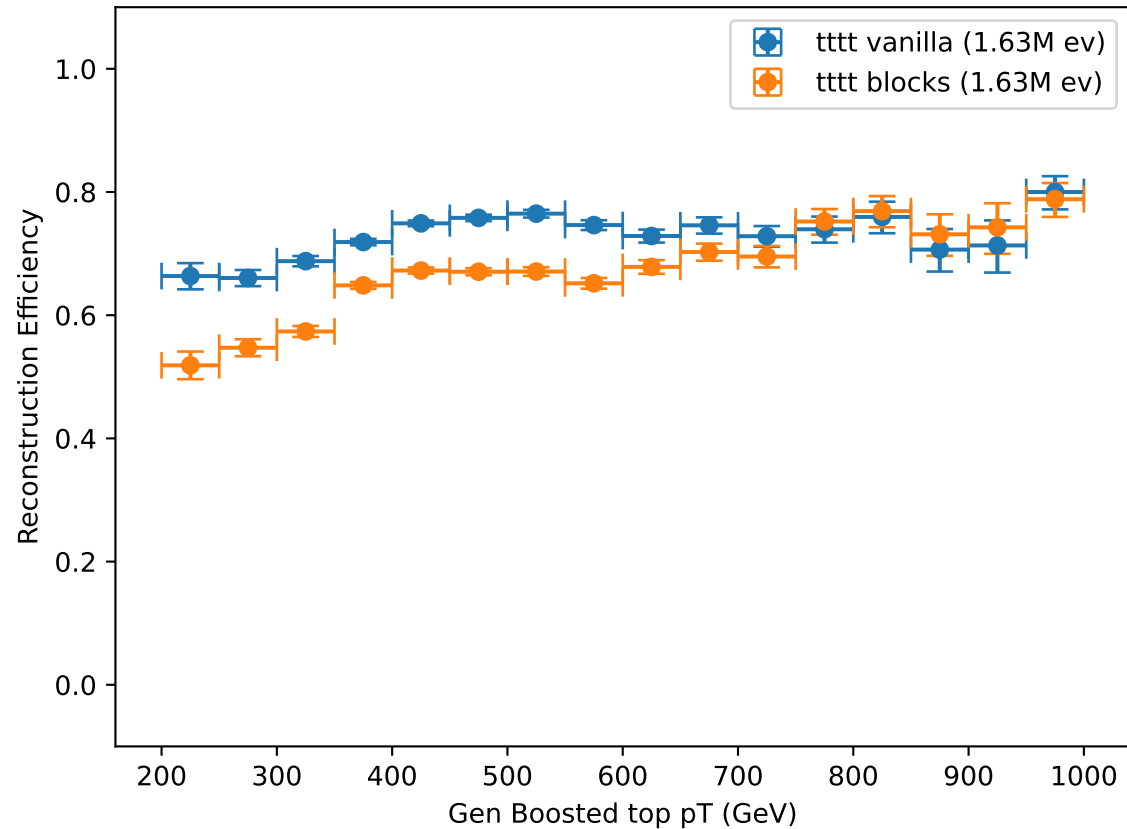
Reconstruction Efficiency vs. Gen Boosted top pT
