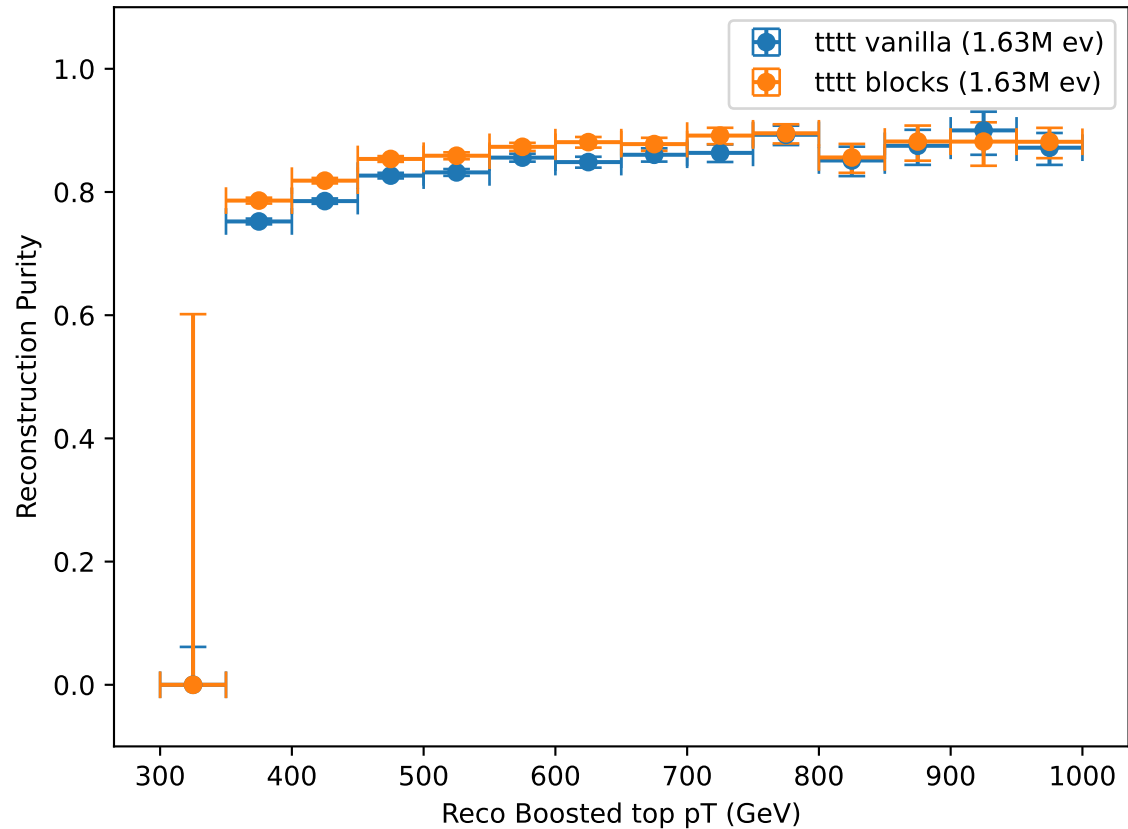
Reconstruction Purity vs. Reco Boosted top pT
