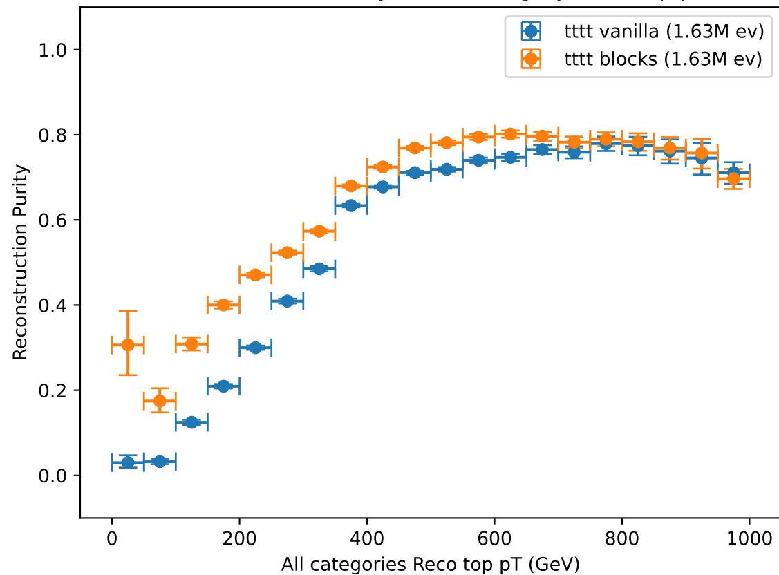
Reconstruction Purity vs. All category Reco top pT
