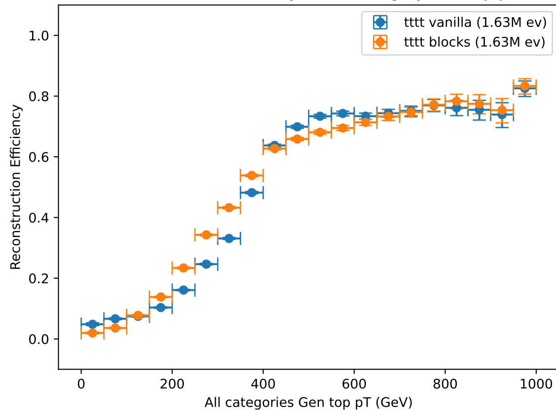
Reconstruction Efficiency vs. All category Gen top pT
